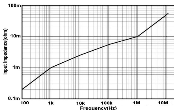
Fig 12.a HCPX8150 Input Impedance-Frequency curve
