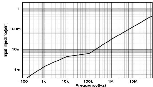
Fig 3.b HCPX8030C Input impedance VS Frequency curve
