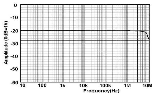
Fig 13.b HCPX8300A Amplitude-frequency Curve
