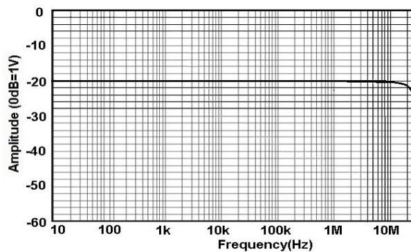
Figure 10.b HCPX8150A Amplitude-Frequency Curve
