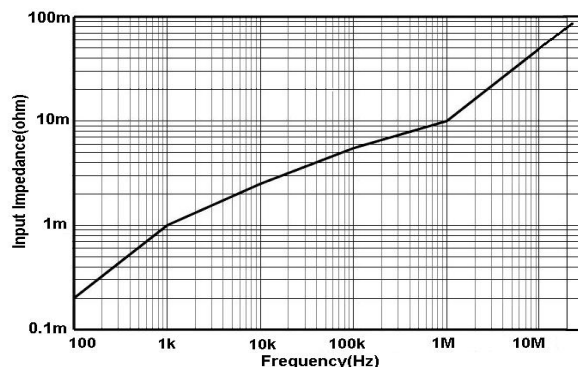
Fig12.b HCPX8150A Input Impedance-Frequency curve
