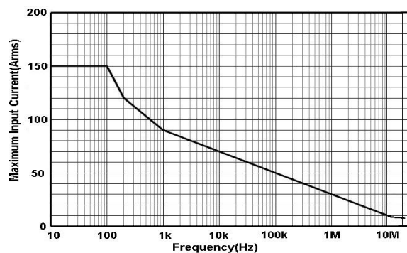
Fig 11.b HCPX8150A Continuous maximum input measurement
