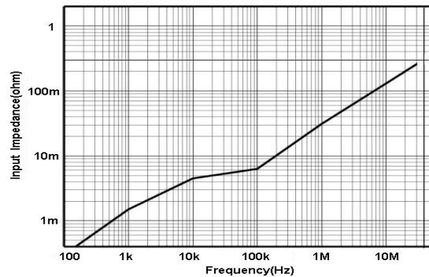
Fig 9 HCPX8070 Input Impedance-frequency curve
