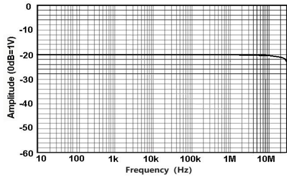
Fig 7 HCPX8070 Amplitude-Frequency Curve
