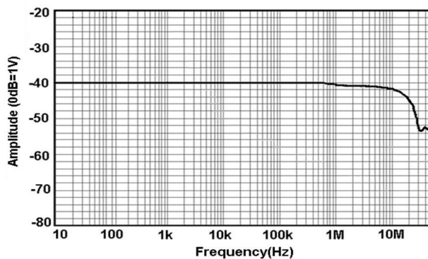
Figure 10.a HCPX8150 Amplitude-Frequency Curve
