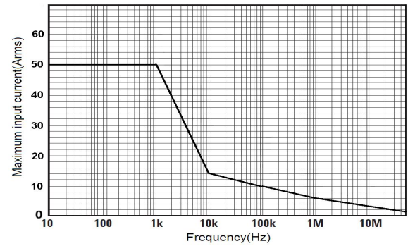
Fig 5 HCPX8050 Continuous maximum input rating
