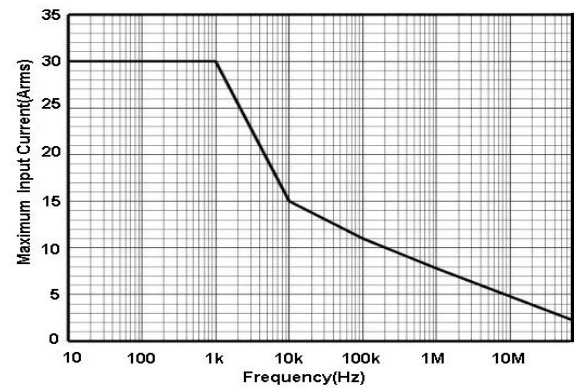
Fig 2.b HCPX8030C Continuous maximum input measurement
