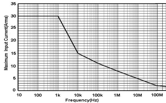
Fig 2.d HCPX8030H Continuous maximum input measurement
